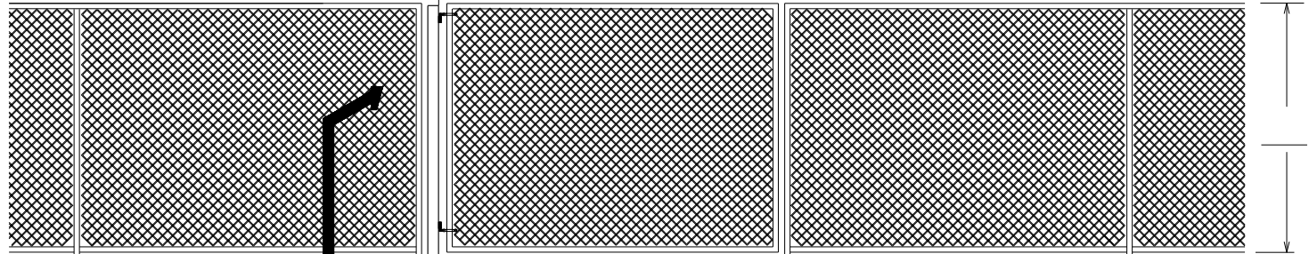
6'-0" HIGH CHAINLINK GATE ( 8'-0" OR LESS WIDE ) EXTERIOR ELEVATION
