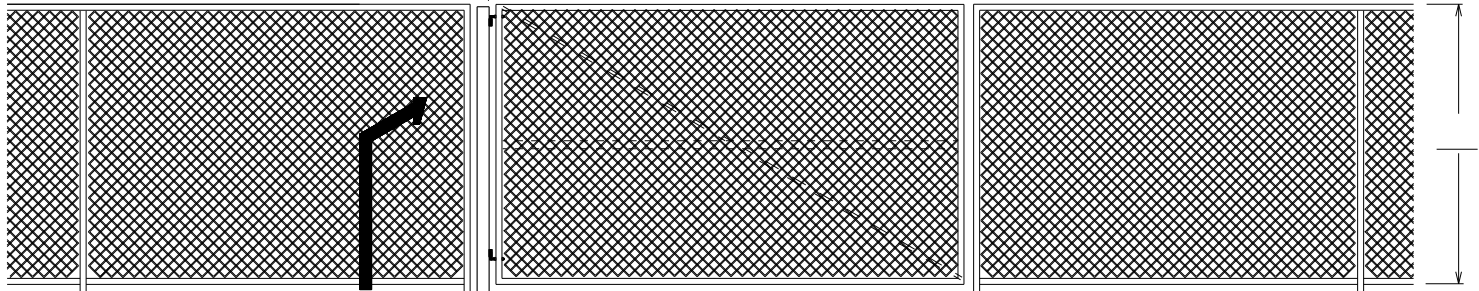
6'-0" HIGH CHAINLINK GATE ( 8'-0" OR MORE WIDE ) EXTERIOR ELEVATION
