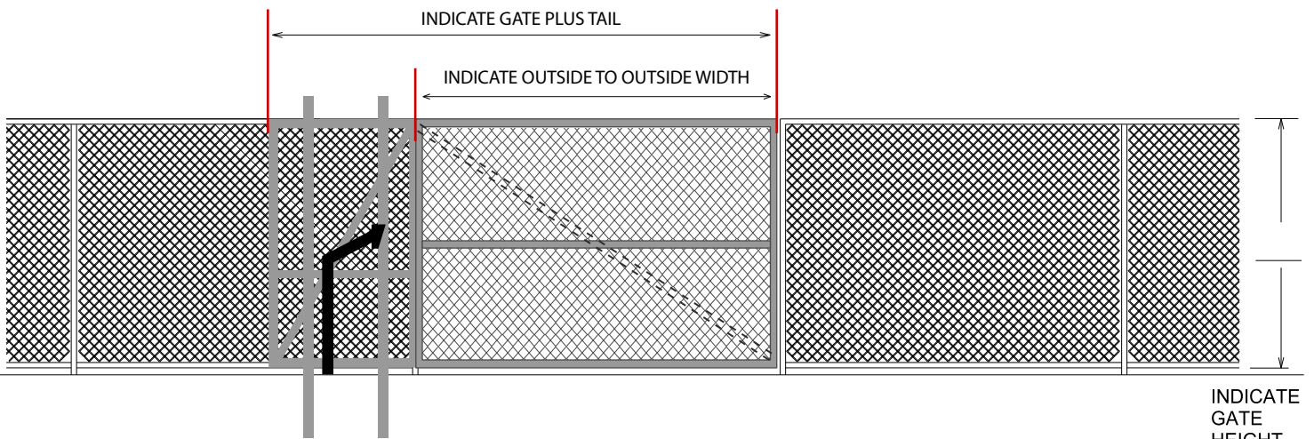
6'-0" HIGH CHAINLINK GATE (8'-0" OR MORE WIDE) EXTERIOR ELEVATION
